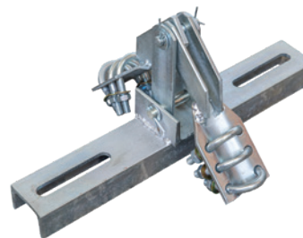
HINGED CONNECTION FOR POLE
